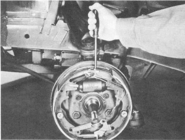
Fig. 16 — Test adjuster with drum off
