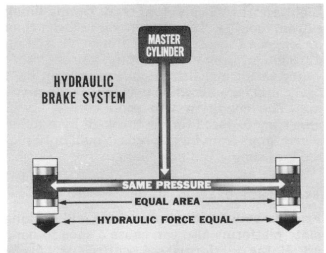
Fig. 5 — Hydraulic force is equal
