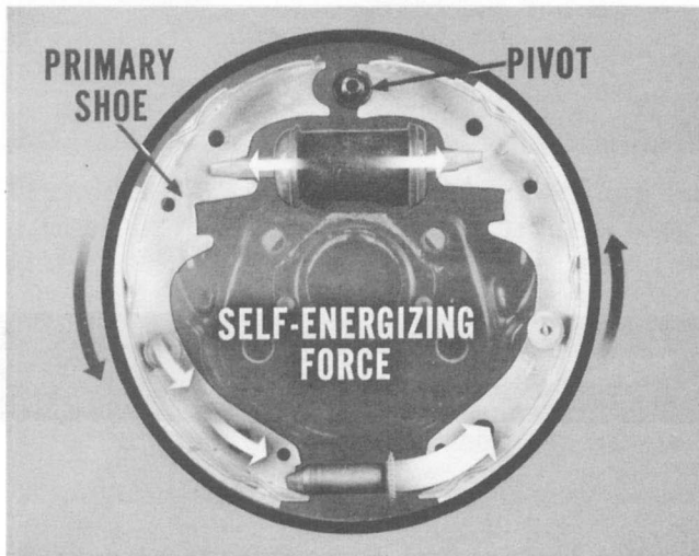
Fig. 2 — Self-energizing action
