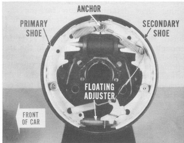
Fig. 1 — Servo-Contact Brake
