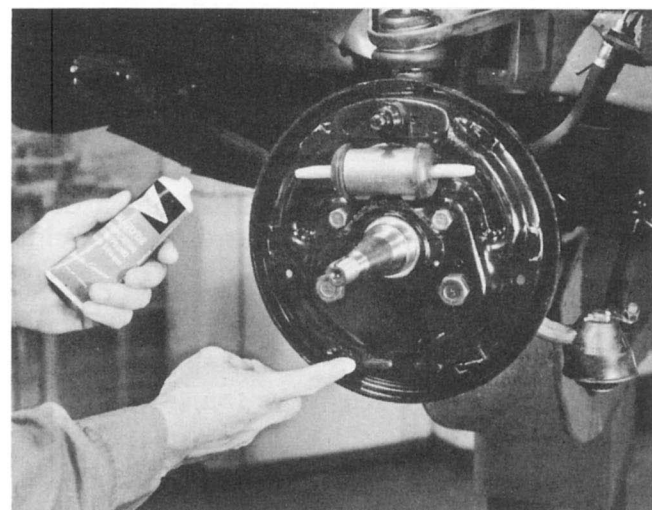
Fig. 7 — Lubricate platforms sparingly
