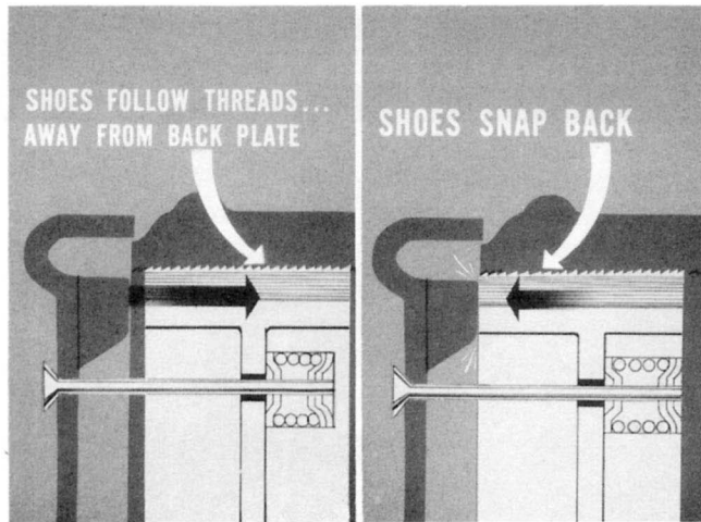
Fig. 10 — Threading causes shoe knock
