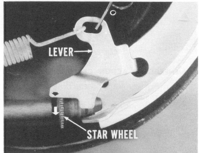
Fig. 4 — Adjuster lever turns star wheel
