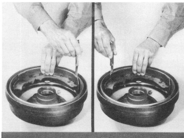
Fig. 14 — Heel-and-toe clearance
