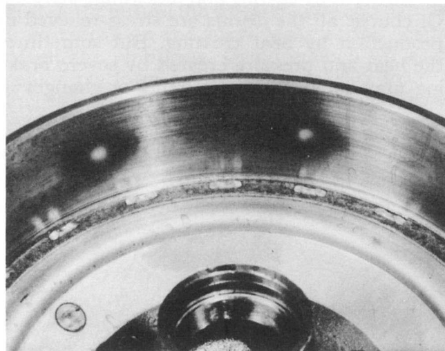
Fig. 9 — Severe heat spot
