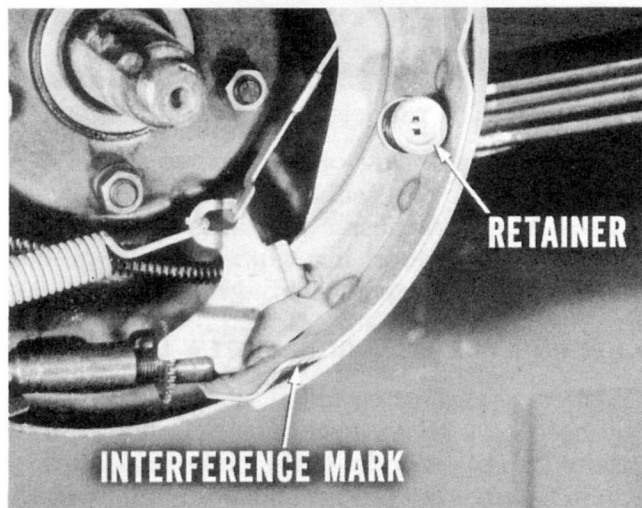
Fig. 11 — Shoe scrape interference mark
