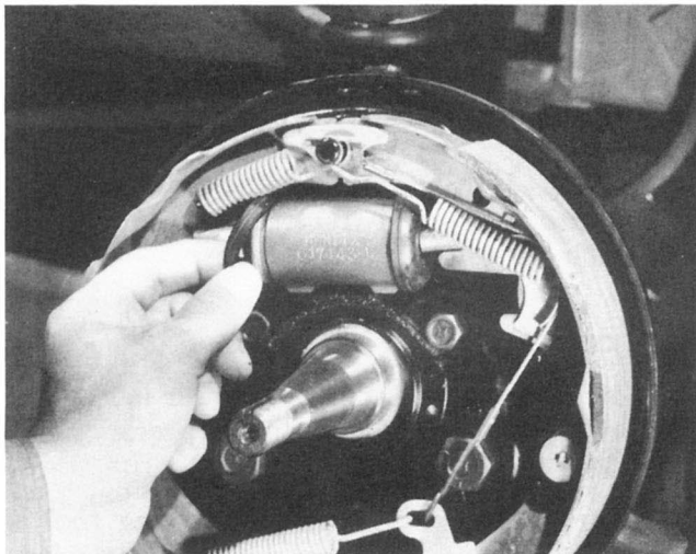
Fig. 13 — Check for wheel cylinder leaks
