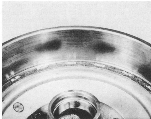
Fig. 8 — "Incipient" heat spot
