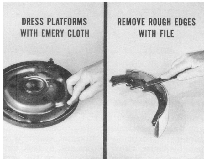
Fig. 6 — Dress down platforms and loops
