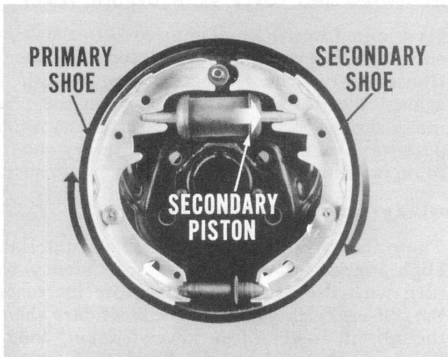
Fig. 3 — Reverse braking action
