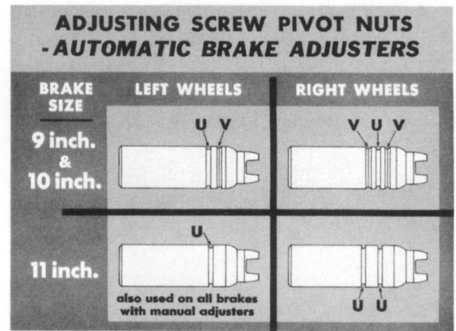
Fig. 20 — Adjuster identification
