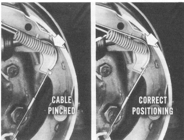
Fig. 17 — Check cable for binding at guide
