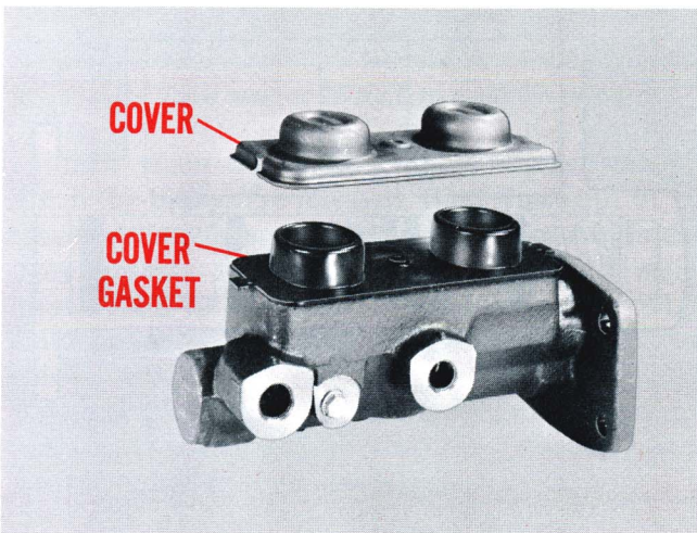
Fig. 10—Cover gasket must keep moisture out
