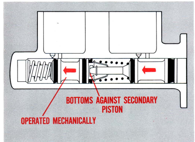
Fig. 8—Hydraulic link is broken
