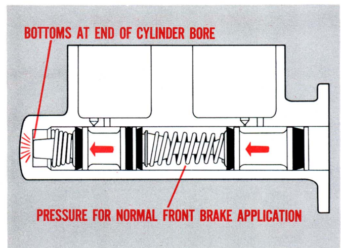
Fig. 9—When secondary bottoms, primary goes to work
