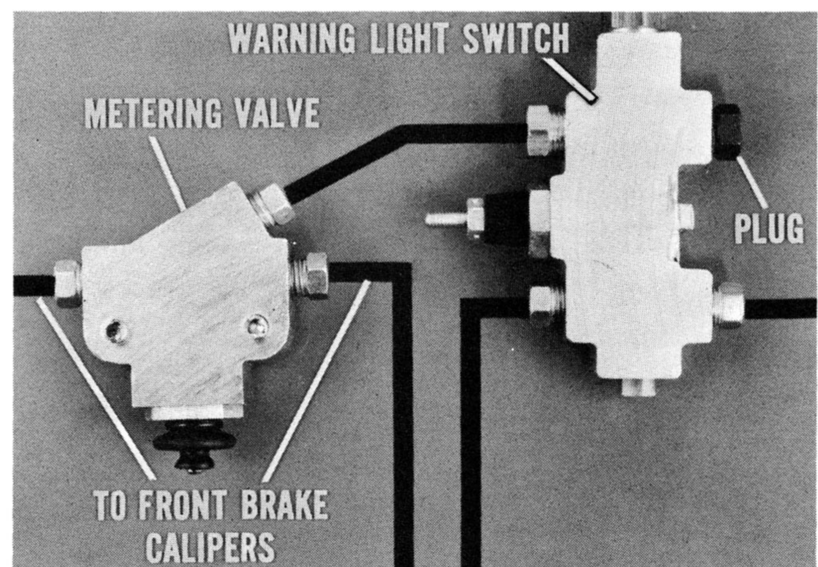
Fig. 27—Metering valve acts as "tee"
