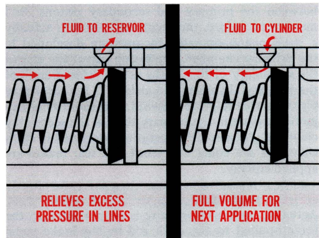
Fig. 5—Compensating ports prevent brake drag
