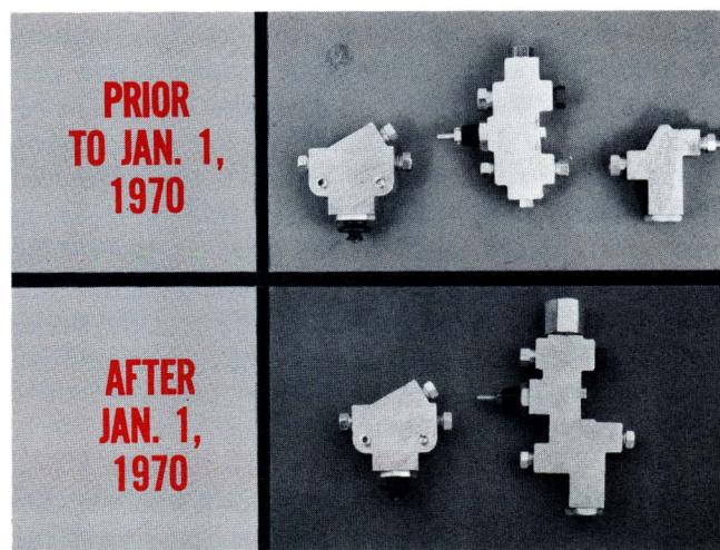
Fig. 16—Switch and proportioning valve combined
