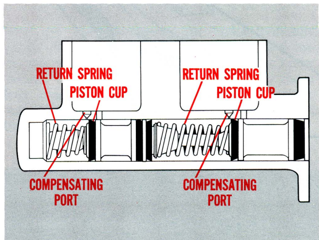
Fig. 2—Springs return piston and brake pedal
