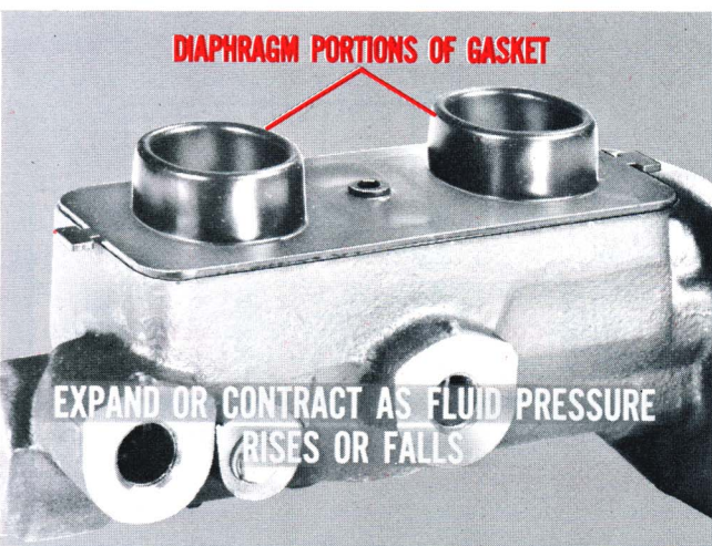
Fig. 11—Cover gasket also acts as a diaphragm
