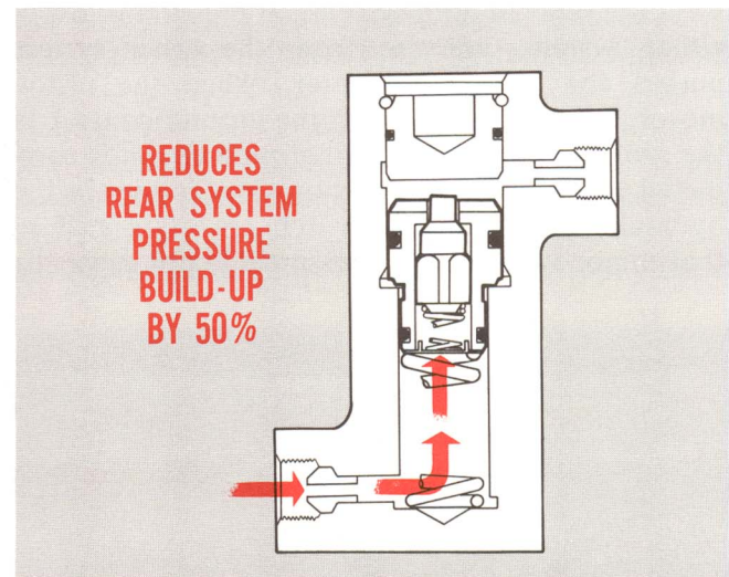
Fig. 21—Pressure is reduced above 300 p.s.i.
