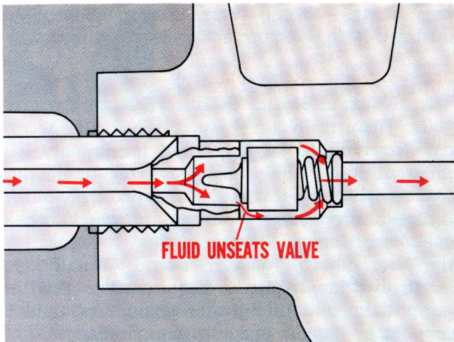
Fig. 4—Valve seats at 15 p.s.i. to maintain pressure
