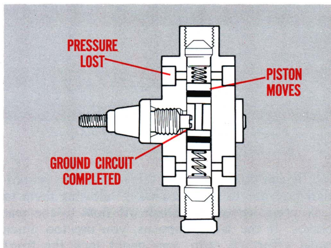
Fig. 17—Minor pressure variations won't move piston
