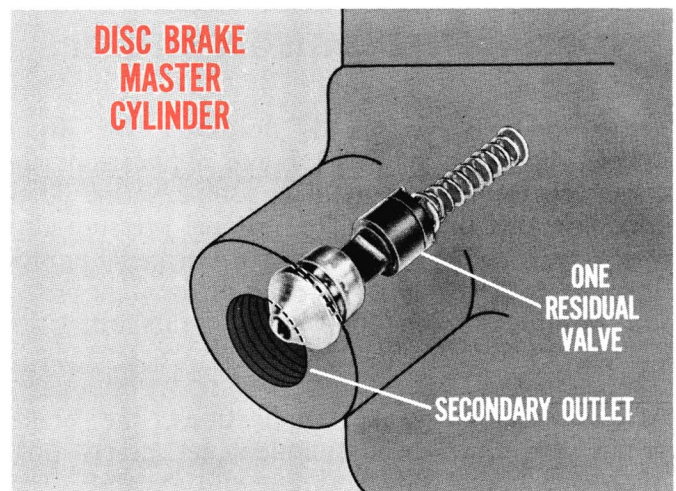
Fig. 3—Residual pressure would make disc brakes drag
